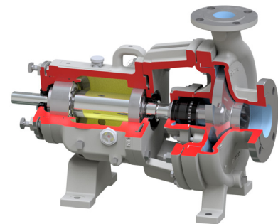
ASME Standard Pump
